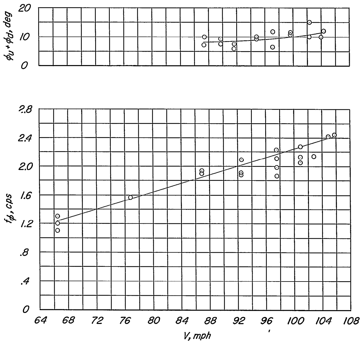
(c) \delta = 8^\circ ; light fighters.
