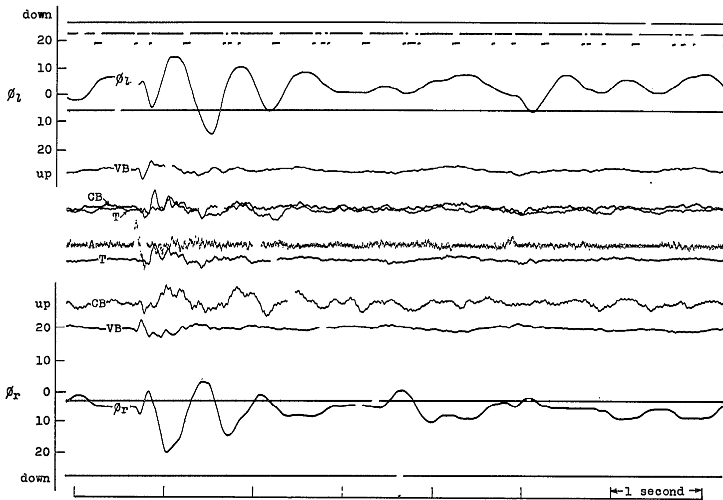
(b) V = 78.3 mph; symmetric excitation.
