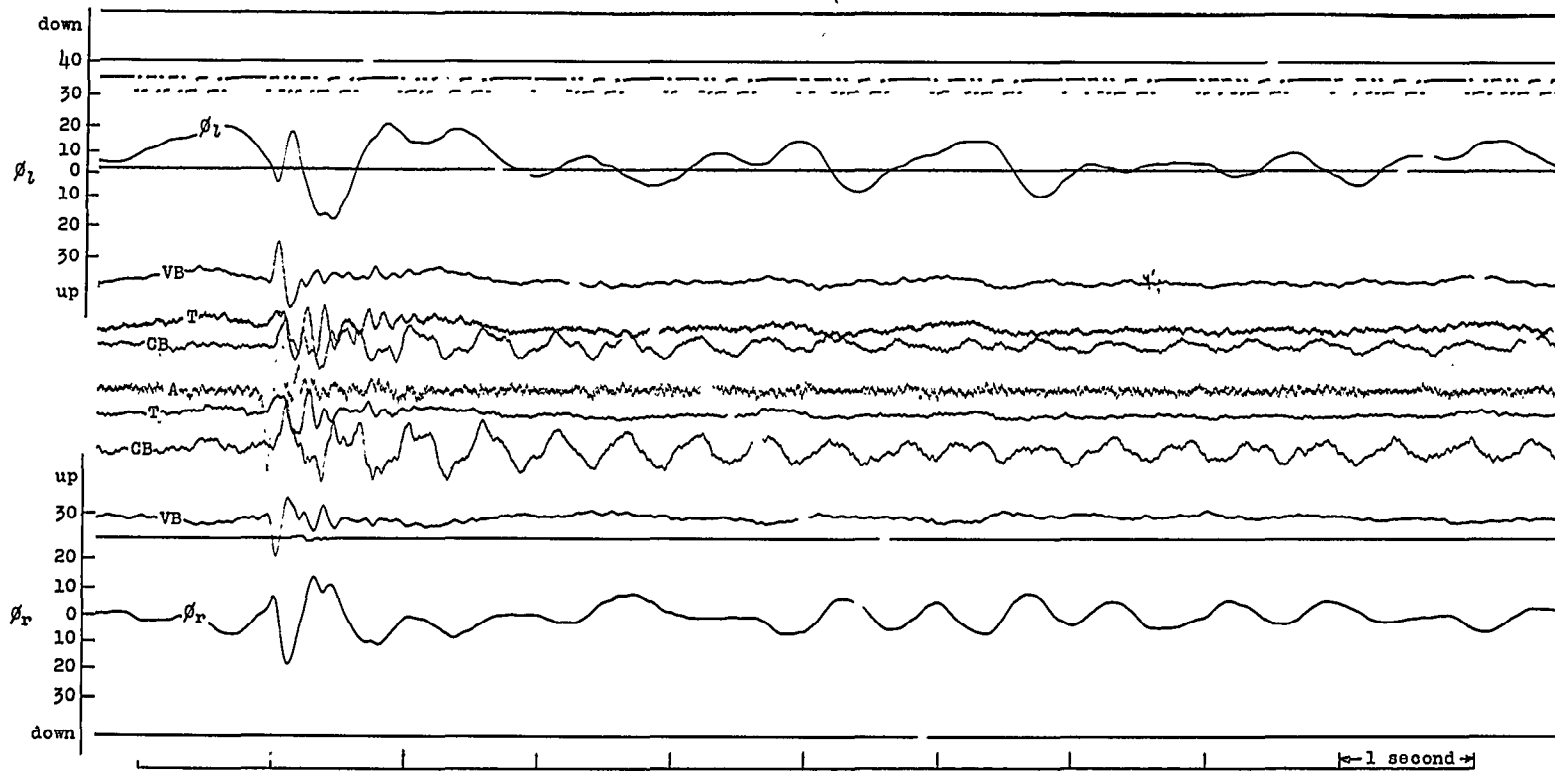
(c) V = 89.7 mph; symmetric excitation.
