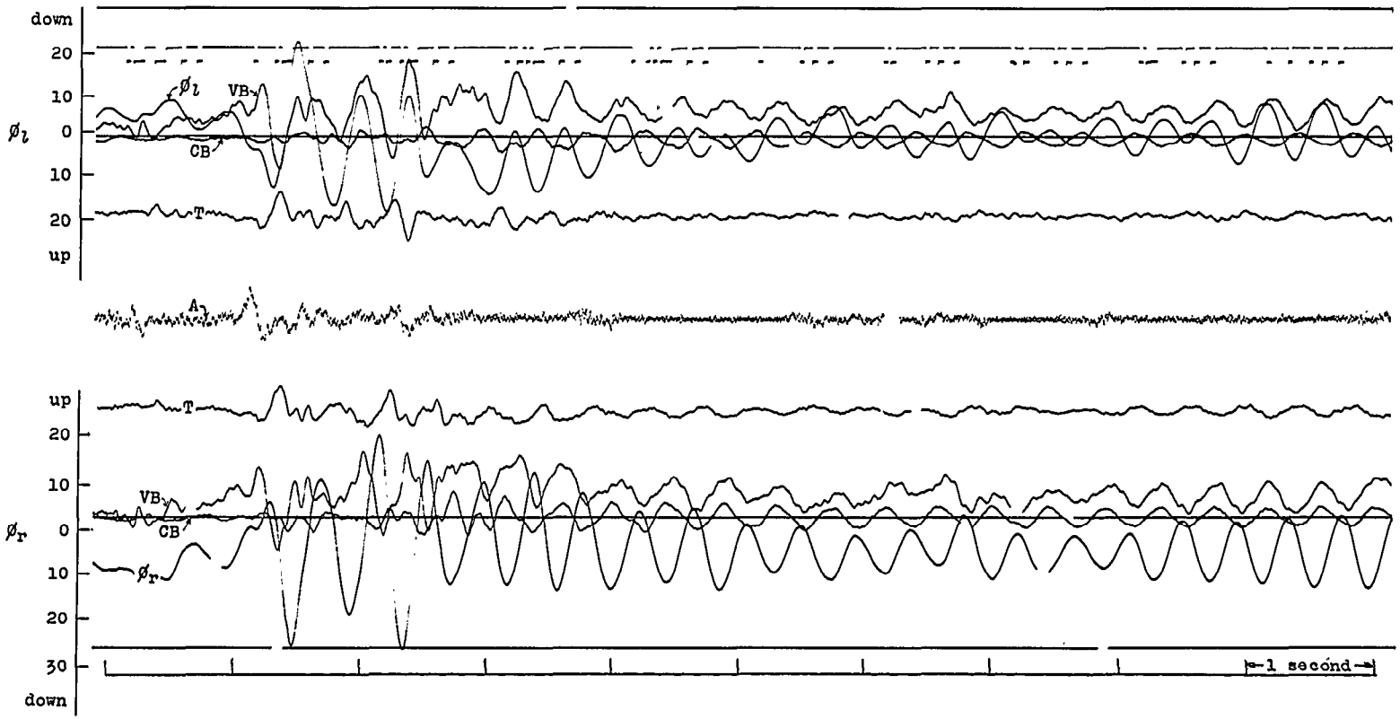
(c) V = 81.7 mph; symmetric excitation.
