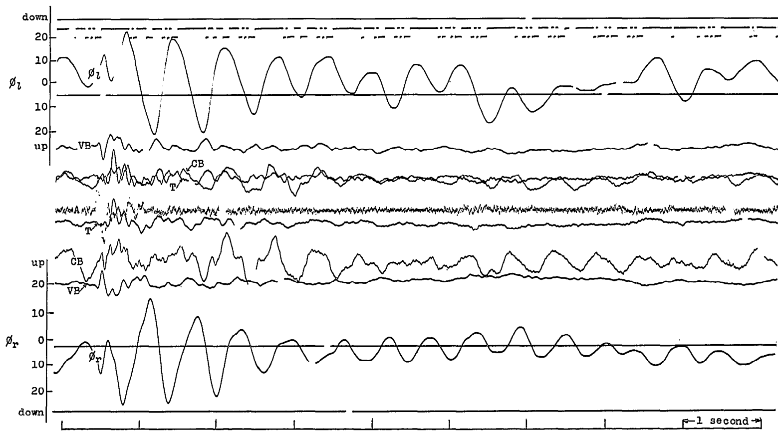
(c) V = 84.0 mph; symmetric excitation.
