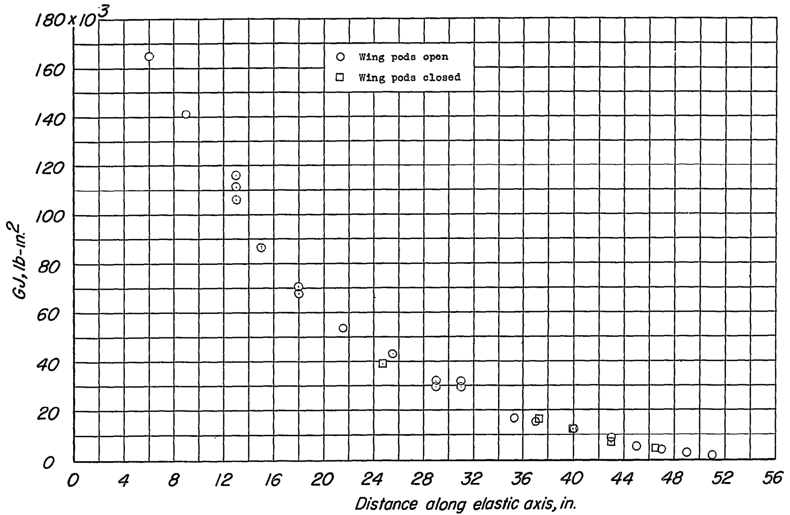
(c) Torsional rigidity.
