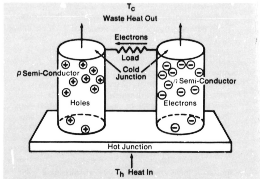
13 When the hot junction of a thermoelectric couple is heated, electrons and holes are driven toward the cold ends of the semiconductor cylinders. Electrons flow through the load and neutralize the positive holes.
