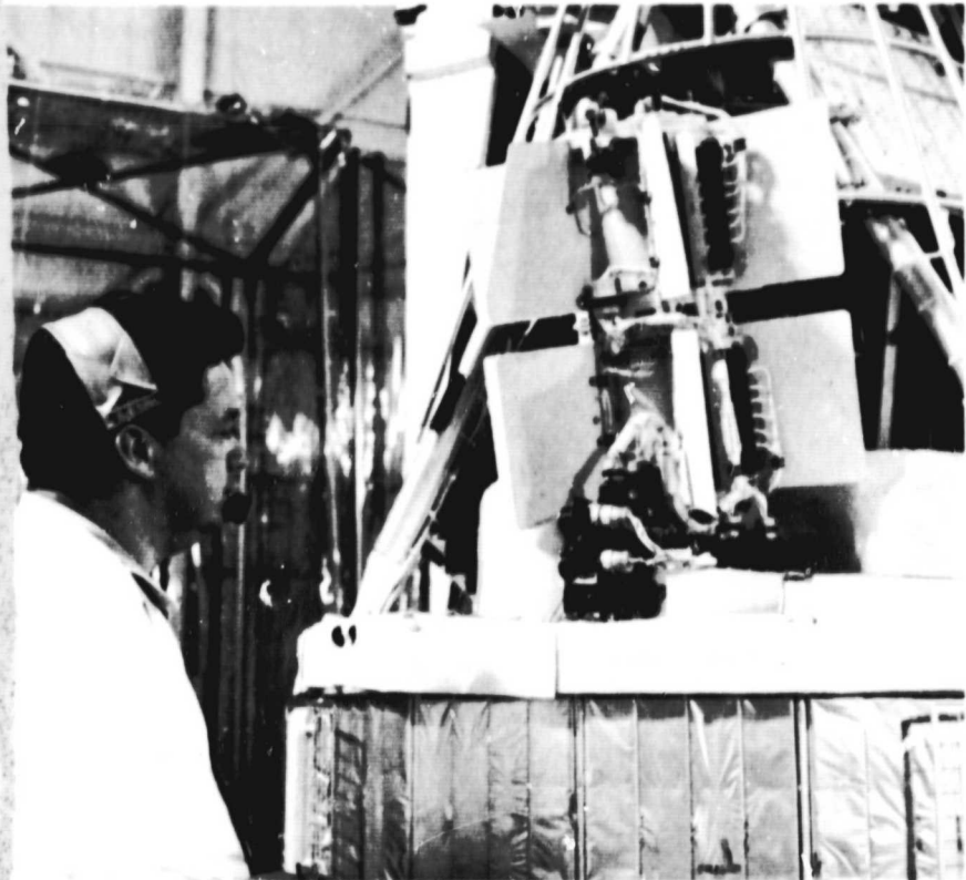
14 Closeup of two SNAP-19's mounted on the Nimbus weather satellite. Note the large fins needed to radiate away waste heat. SNAP-19 generated about 25 watts of electric power and weighed about 30 pounds.
