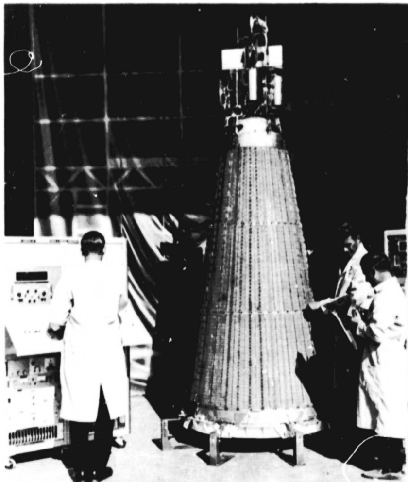
16 SNAP-10A. The reactor is perched on the top of the cone that forms the radiator surface. During launch, the whole power plant was protected by a shroud.
