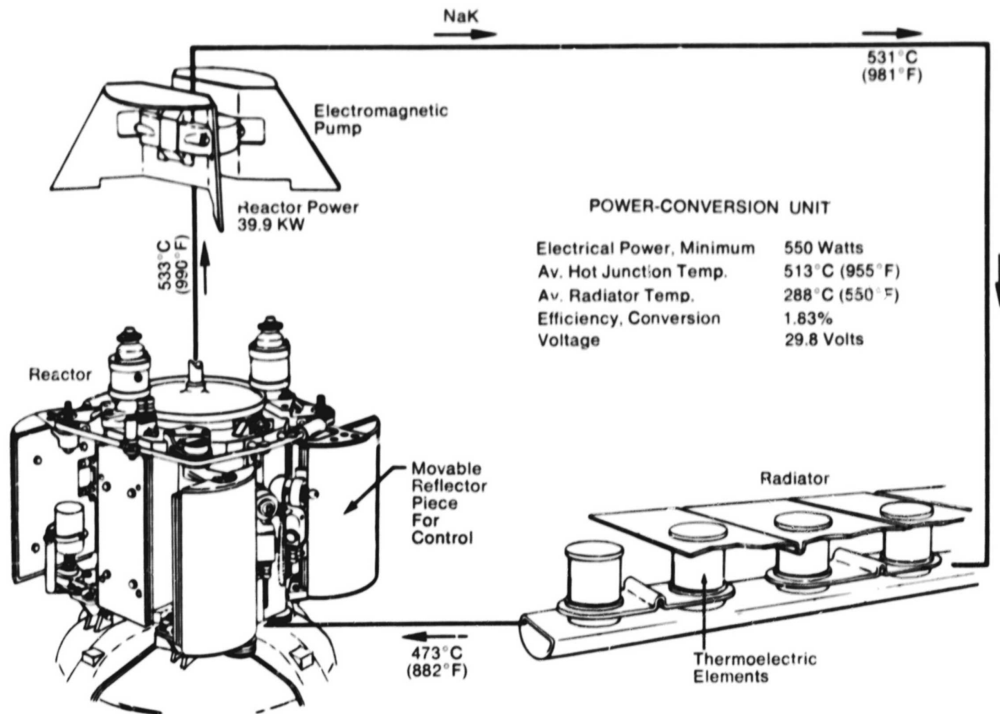
17 Schematic of the SNAP-10A reactor-thermoelectric power plant.
