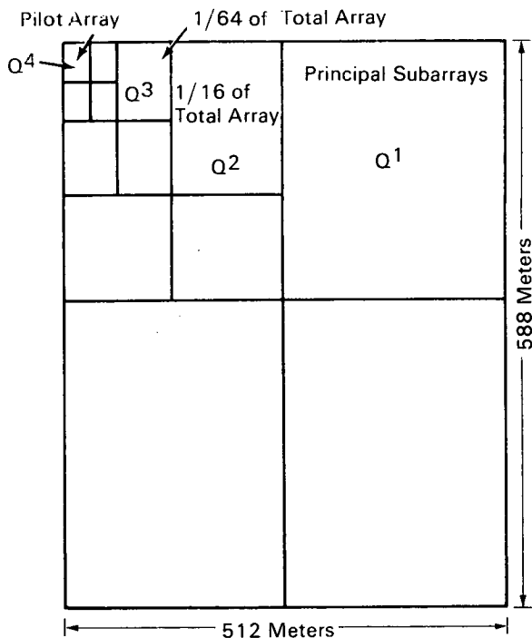
Receiving Antenna Array Layout
