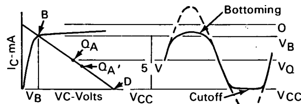
Figure 2. Load Line (Left) and Wave Form
