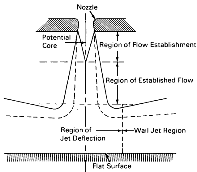
Characteristic Regions in Impinging Jet Flow
