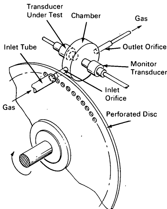
Inlet-Area-Modulated Sinusoidal Pressure Generator
