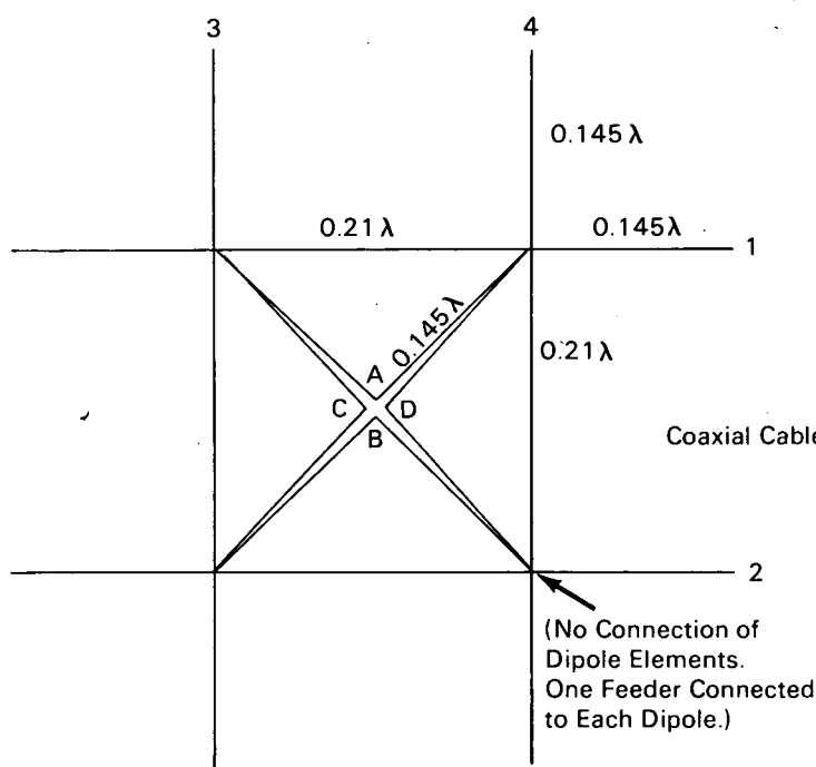
HALF-WAVE DIPOLE ELEMENTS
