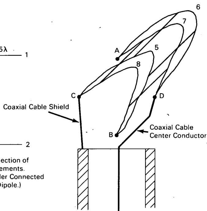
EXPLODED VIEW OF FEED AND PHASING SYSTEM
