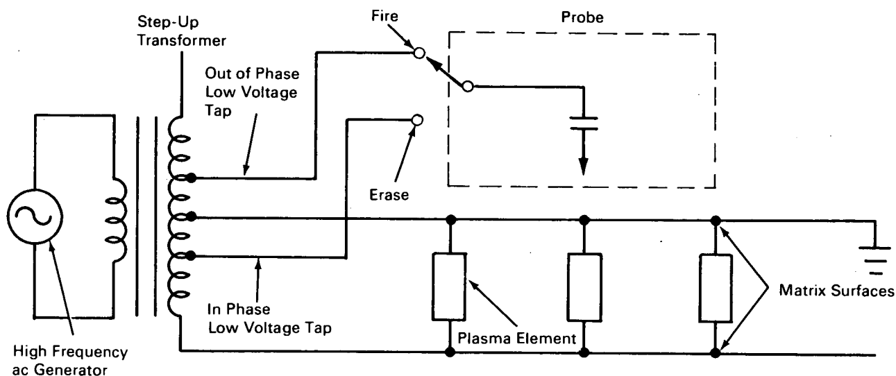
Figure 1. Probe Drive
