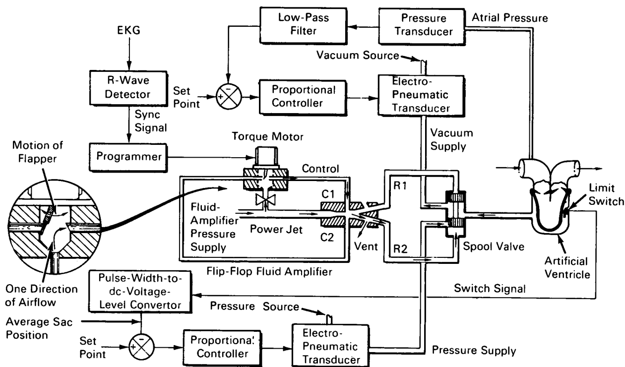
Control System for an Artificial Heart: Diagrammatic
