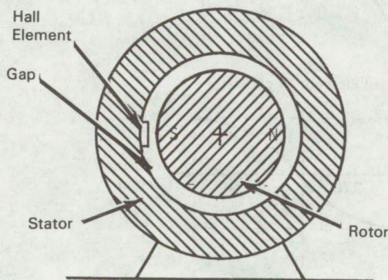
Figure 1. Element Location
