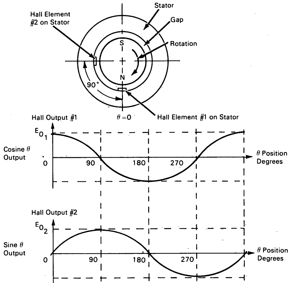
Figure 2. Sine and Cosine Outputs During Rotor Movement
