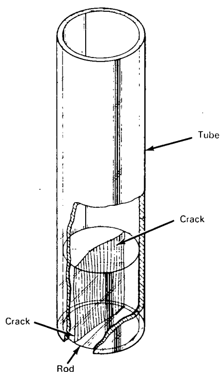
Cracked Rod Reassembled within Tube
