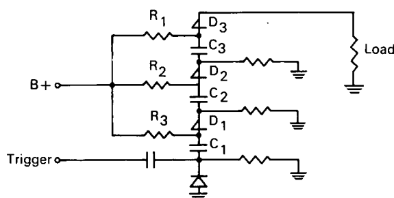
CONVENTIONAL CIRCUIT
