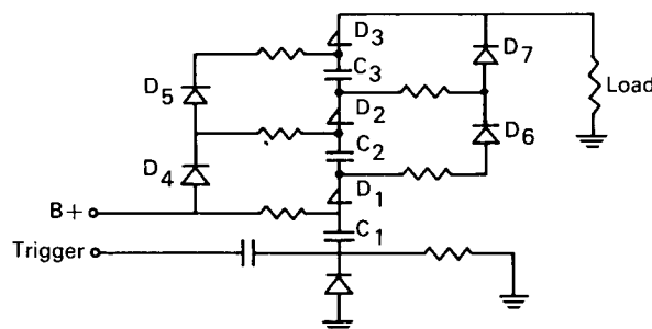
IMPROVED CIRCUIT
