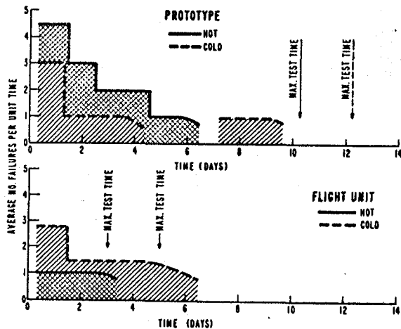
Figure 5. Summary of Spacecraft Failures versus Time in Thermal-Vacuum Tests.
