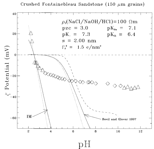
Figure 13. The \zeta potential, inferred from streaming potential measurements using crushed Fontainebleau sandstone, as a function of pH for NaCl/HCl/NaOH solutions. Diamonds correspond to measurements with an electrolyte resistivity of 100 \Omega m. Triangles correspond to measurements for which the electrolyte resistivity is controlled by the pH and cannot be maintained at 100 \Omega m. The measurement experimental errors are of the size of the symbols. The lines correspond to the predictions of a simplified one-layer model [Revil and Glover, 1997]. The solid line corresponds to the default parameters indicated. The dotted line refers to the related Stern plane potential. The dashed line correspond to the parameters of the three-layer model indicated in Figure 11. The prediction from Ishido and Mizutani [1981] is also shown for comparison (IM).
