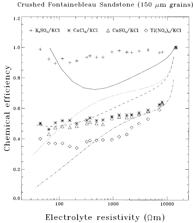
Figure 18. The streaming potential chemical efficiency as a function of electrolyte resistivity for several salt solutions with \text{pH} = 5.7 . The measurement experimental errors are of the size of the symbols. The lines correspond to the predictions of the three-layer model [Davis et al. , 1978] with the parameters indicated in Table 1, from top to bottom \text{K}_2\text{SO}_4 , \text{CaCl}_2 , \text{CaSO}_4 , and \text{Tl}(\text{NO}_3)_3 .
