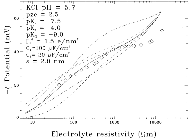
Figure 7. The \zeta potential, inferred from streaming potential measurements using crushed Fontainebleau sandstone, as a function of electrolyte resistivity for KCl solutions with pH = 5.7. The measurement experimental errors are of the size of the symbols. The lines correspond to the predictions of the three-layer model [Davis et al. , 1978]. The solid line correspond to the default parameters indicated. The dotted line refers to the related Stern plane potential. The dashed lines correspond to pK_{K^+} increased or decreased by 1. When K_{K^+} is increased, the absolute value of the \zeta potential is decreased. The dash-dotted lines correspond to pK_{Cl} increased or decreased by 1. When K_{Cl} is increased, the absolute value of the \zeta potential is increased.
