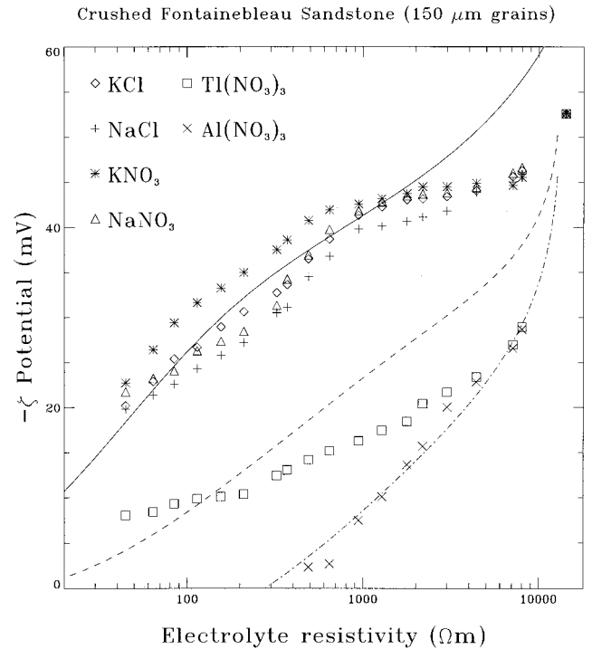
Figure 20. The \zeta potential, inferred from streaming potential measurements using crushed Fontainebleau sandstone, as a function of electrolyte resistivity for several salt solutions with \text{pH} = 5.7 . The results for \text{Na}^+ and \text{K}^+ are compared for two anions, and two examples of trivalent ions are given. The lines correspond to the predictions of the three-layer model [Davis et al. , 1978], from top to bottom KCl, \text{TI}(\text{NO}_3)_3 , and \text{Al}(\text{NO}_3)_3 . The inferred values of the equilibrium constants are pK_{\text{TI}} = 5.6 (Table 1) and pK_{\text{Al}} = 3.7 .
