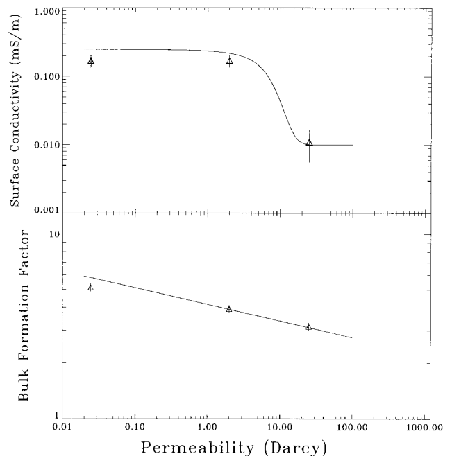
Figure 21b. Surface conductivity and bulk formation factor as a function of permeability. The three experimental measurements are compared with the ad hoc model (solid line) described in the text and used to correct for surface conductivity in Figure 21a.
