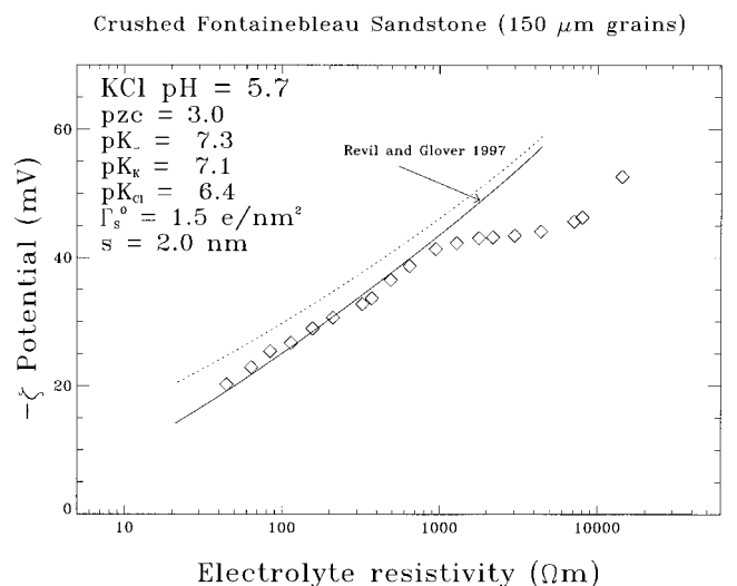
Figure 9. The \zeta potential, inferred from streaming potential measurements using crushed Fontainebleau sandstone, as a function of electrolyte resistivity for KCl solutions with pH = 5.7. The measurement experimental errors are of the size of the symbols. The lines correspond to the predictions of a simplified one-layer model [Revil and Glover, 1997]. The solid line corresponds to the default parameters indicated. The dotted line refers to the related Stern plane potential.
