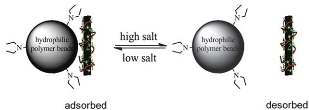
Fig. 5 Anion-exchange chromatography separation of DNA-SWCNTs. Anion exchange columns are packed with micro-sized polymer or silica beads that are surface-grafted with positively charged functional groups. DNA-SWCNTs injected into the column can be either adsorbed on the beads or remain free, depending on the concentration and chemical identity of the salt in the mobile phase. The equilibrium is also dependent on SWCNT structure, leading to fractionation of DNA-SWCNTs when they are eluted from the column by a salt gradient. By tailoring specific ssDNA strands to form ordered structures only on a specific (n,m) SWCNT surface, preferential adsorption and retention can be achieved leading to single-chirality samples.
