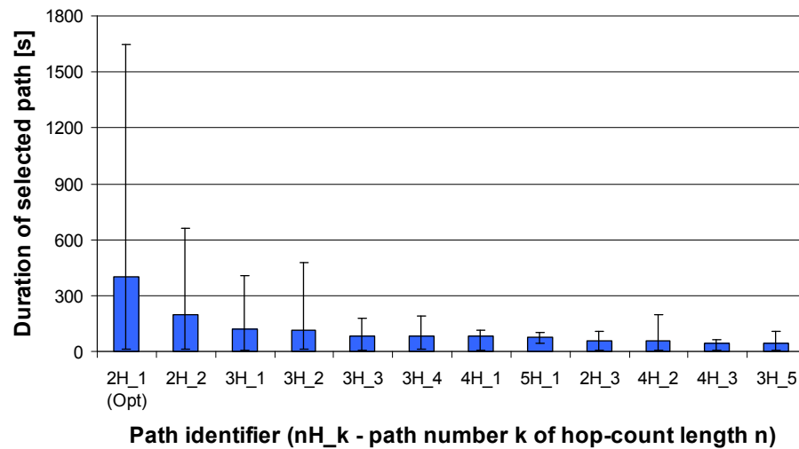
Figure 3.7 : Durations and hop-count lengths of paths selected by the reference node 17. Presented are average, minimal, and maximal durations.
