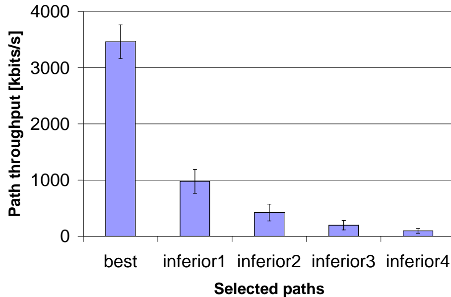
Figure 3.8 : Persistence of throughputs of isolated paths connecting the reference node 17 to the GW. Presented are average values and standard deviations.
