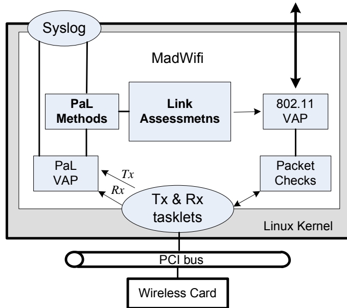
Figure 2.7 : PaL implementation.
