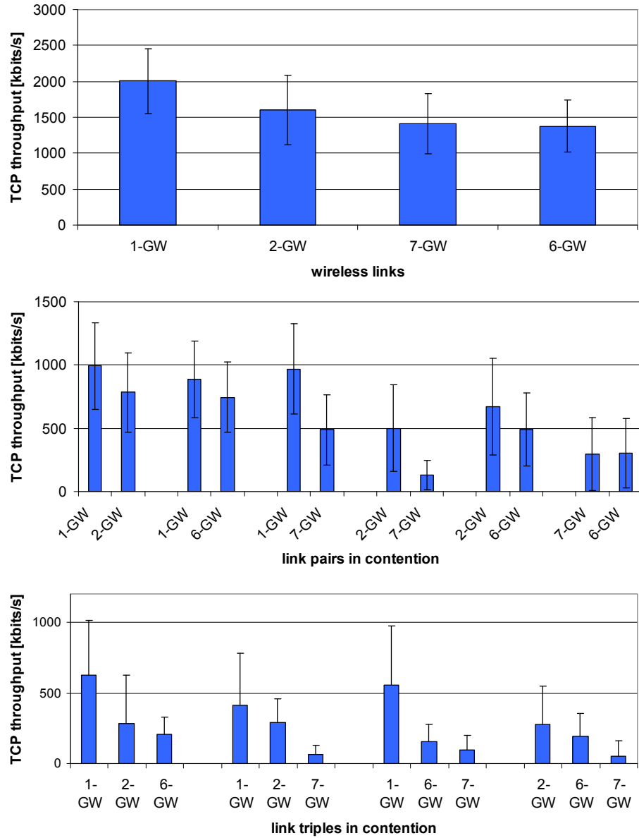
Figure 3.9 : Persistence of throughputs of contending links. Presented are average values and standard deviations.
