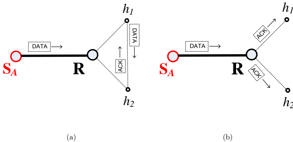
Figure 2.5 : Sender's S_A identification of hidden terminal activity: (a) Blind identification, and (b) Identification by ACK analysis.
