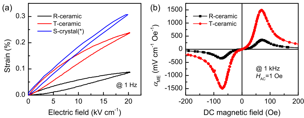
FIG. 4. (a) Strain vs. electric field curves of randomly oriented ceramic (R-ceramic), \langle 001 \rangle textured ceramic (T-ceramic), and \langle 001 \rangle single crystal (S-crystal). (b) Magnetoelectric (ME) voltage coefficients ( \alpha_{ME} ) of random and textured PMN-PZT ceramics.
