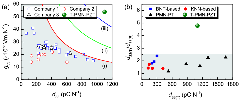
FIG. 1. (a) Comparison of g_{33} and d_{33} values of various piezoelectric ceramics (Ref. 5). Different colored lines (i), (ii), and (iii) indicate the plots of g_{33} \cdot d_{33} = c function; (i) c = 16500 \times 10^{-15} \text{ m}^2 \text{ N}^{-1} , (ii) c = 30\,000 \times 10^{-15} \text{ m}^2 \text{ N}^{-1} , and (iii) c = 50\,000 \times 10^{-15} \text{ m}^2 \text{ N}^{-1} . (b) Comparison of d_{33(T)}/d_{33(R)} ratio vs. d_{33(T)} of various textured piezoelectric ceramics. The d_{33(T)} and d_{33(R)} represent d_{33} of textured ceramic and that of randomly oriented counterpart, respectively. BNT and KNN represent (\text{Bi}_{1-x}\text{Na}_x)\text{TiO}_3 and (\text{K}_{1-x}\text{Na}_x)\text{NbO}_3 compositions, respectively.
