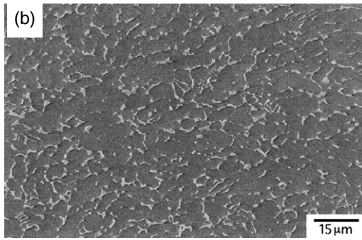
(b) equiaxed [24]
