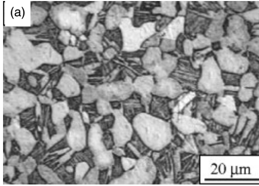
(a) bimodal [10]
