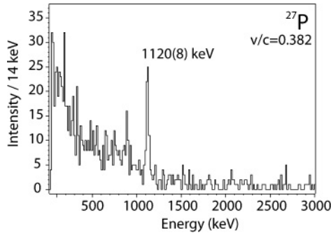
FIG. 5. \gamma -ray spectrum detected in coincidence with ^{27}\text{P} . The 1120-keV level is populated to 18(3)% in the one-proton knockout from ^{28}\text{S} . According to the shell model, one would expect 40%. The discrepancy is most likely explained by the fact that this level is unbound by 260 keV and the \gamma -ray decay will be in strong competition with proton emission. The 3/2^+ state was previously reported at 1199 keV from particle spectroscopy [44].
