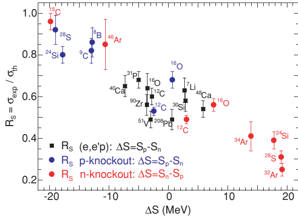
FIG. 6. (Color online) Reduction of the measured nucleon knockout cross sections (spectroscopic strength) relative to theoretical values as a function of the difference in separation energies of the two nucleon species, \Delta S (see text). The data points are from Refs. [5,13–16,19,24]. Those from the present work, labeled ^{24}\text{Si} and ^{28}\text{S} , appear on the extreme left- and right-hand sides of the figure. Only experimental uncertainties are included.
