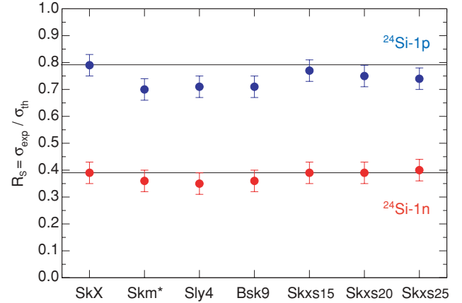
FIG. 7. (Color online) Deduced values of R_s for the reactions ^9\text{Be}(^{24}\text{Si}, ^{23}\text{Al})\text{X} and ^9\text{Be}(^{24}\text{Si}, ^{23}\text{Si})\text{X} as obtained using different Skyrme parametrizations as input to the HF calculations used for the reaction methodology. The R_s factors obtained when using the \text{Skm}^* , \text{Sly4} , \text{Bsk9} , \text{Skxs15} , \text{Skxs20} , and \text{Skxs25} interactions agree within the quoted uncertainties on the value deduced using the \text{SkX} Skyrme parametrization used here. The \text{SkX} values are indicated by the horizontal lines.
