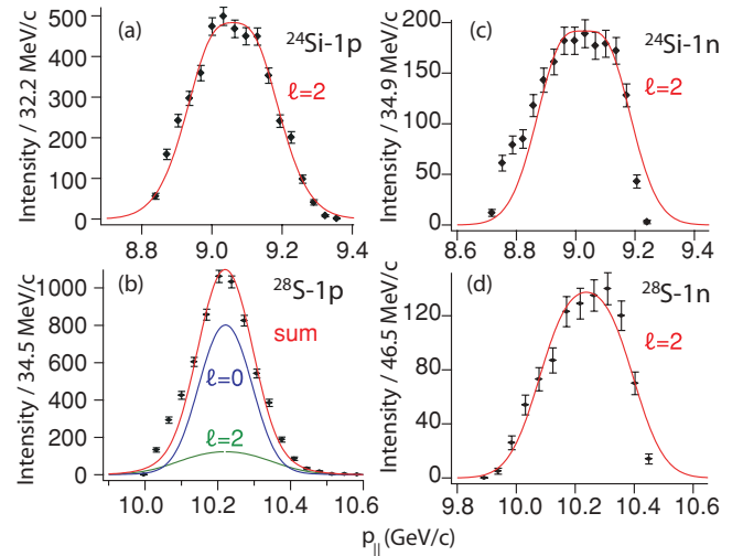
FIG. 4. (Color online) Longitudinal momentum distributions of the knockout residues in the reactions (a) {}^9\text{Be}({}^{24}\text{Si}, {}^{23}\text{Al})\text{X} , (b) {}^9\text{Be}({}^{28}\text{S}, {}^{27}\text{P})\text{X} , (c) {}^9\text{Be}({}^{24}\text{Si}, {}^{23}\text{Si})\text{X} , and (d) {}^9\text{Be}({}^{28}\text{S}, {}^{27}\text{S})\text{X} . Calculated shapes are superimposed, pure \ell = 2 momentum distributions for (a), (c), and (d) and the scaled sum of \ell = 0 (80%) and \ell = 2 (20%) for (b).
