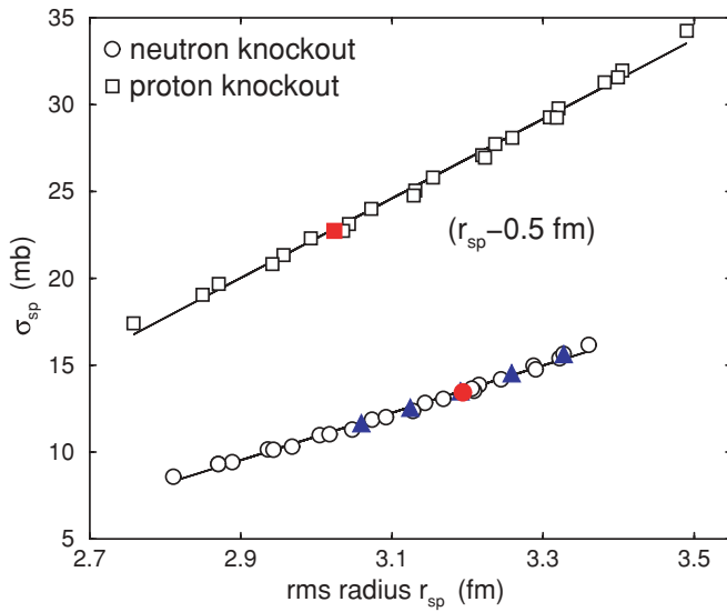
FIG. 2. (Color online) Single-particle cross sections \sigma_{sp} to the ^{23}\text{Si} and ^{23}\text{Al} ground states, assuming 1d_{5/2} neutron- (circles) and 1d_{5/2} proton-removal (squares) from ^{24}\text{Si} at 85.3 MeV/nucleon. Each point assumes different radius r_0 and diffuseness a_0 parameters for the potential used to calculate the nucleon bound-state wave function. The r_{sp} values used in the physical calculations are shown by the filled (red) symbols. Cross sections indicated by blue triangles also include a nonlocality \beta \neq 0 . Note that the proton orbital radii have been displaced to smaller values ( r_{sp} - 0.5 fm) for display purposes.
