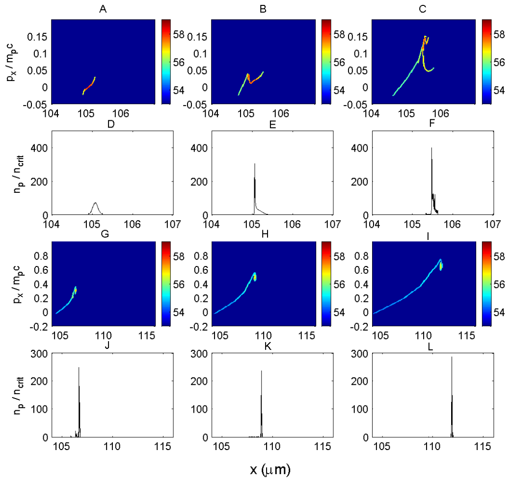
Figure 2. (A–C and G–I) Proton \log_{10} p_x - x phase space plots in the standard run. (D–F and J–L) Proton density ( n_p/n_{\text{crit}} ) profiles in the standard run. Times are: A and D = 20 fs, B and E = 40 fs, C and F = 60 fs, G and J = 80 fs, H and K = 100 fs and I and L = 120 fs. Note the changes in scale. It can be seen that, after 60 fs, the foil moves as a whole with only a very small amount of material being left as trailing mass.
