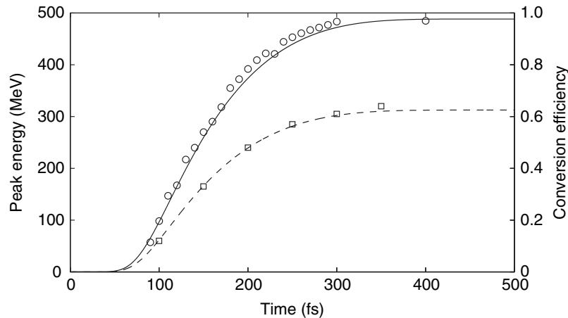
Figure 3. Comparison of semi-analytic model (solid line) with peak proton energy in the standard run (circles). Conversion efficiency also shown for both the model (dashed line) and standard run (squares).
