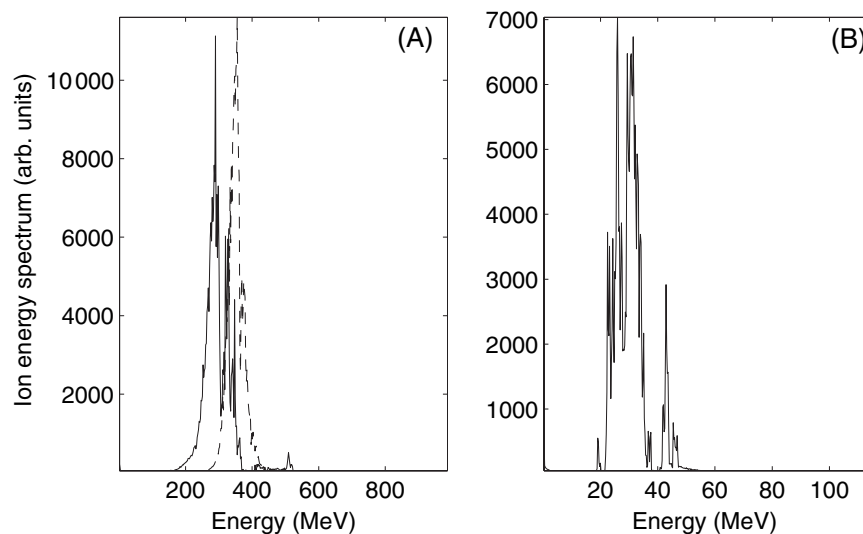
Figure 5. Left panel: C 6+ energy spectra in 1 : 1 C 6+ : H + simulations (solid) and pure C 6+ simulation (dashed). Right panel: proton energy spectrum in 1 : 1 C 6+ : H + simulation.
