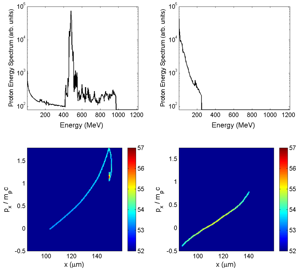
Figure 1. Top left panel: proton energy spectrum after 400 fs in the standard run. Bottom left panel: \log_{10} p_x - x proton phase space at 400 fs in standard run. Top right panel: proton energy spectrum for identical parameters but with linear polarization. Bottom right panel: \log_{10} p_x - x proton phase space at 400 fs in linear polarization run. In the case of circular polarization the foil is accelerated as a whole, leading to a narrow energy spectrum, whereas in the case of linear polarization the foil violently decompresses and produces a broad energy spectrum.
