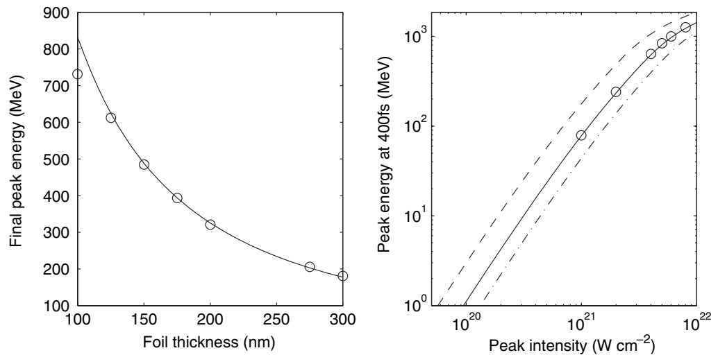
Figure 4. Peak proton energy against foil thickness (left panel) and peak intensity (right panel) in both PIC simulations (circles) and semi-analytic model (lines). Dashed: 150 nm, solid: 250 nm and dash-dot: 350 nm foil thickness in right panel.
