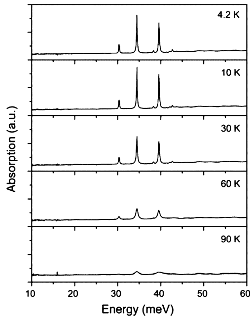
Fig. 13. Terahertz absorption from a boron-doped silicon wafer with temperature. The wafer has a resistivity of 10\text{--}20\ \Omega\text{-cm} , giving a boron concentration of \sim 1 \times 10^{15}\ \text{cm}^{-3} .
