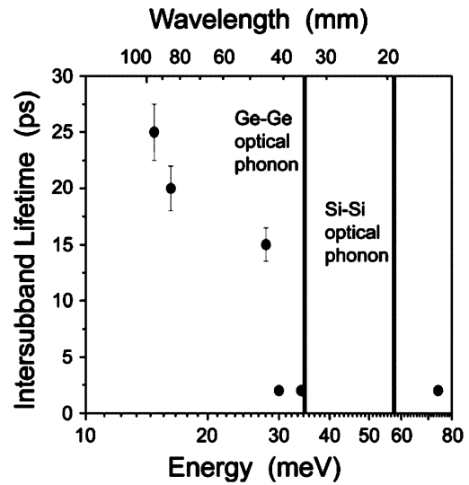
Fig. 7. Plot of intersubband lifetime for an intrawell LH1-to-HH1 transition against both energy ( bottom axis ) and wavelength ( top axis ). The three points above 30 meV are resolution limited in the experiment so that the values are below the probe width of 2 ps.
