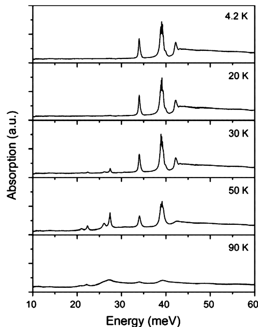
Fig. 14. Terahertz absorption from a phosphorus-doped silicon wafer with temperature. The wafer has a resistivity of 0.3\ \Omega\text{-cm} , giving a phosphorus concentration of 1.5 \times 10^{16}\ \text{cm}^{-3} .
