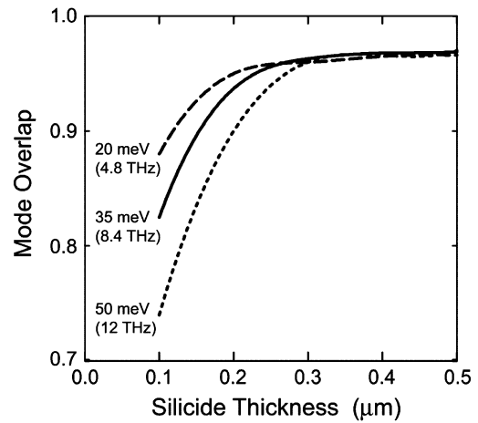
Fig. 9. Plot showing the mode overlap against buried silicide (WSi 2 ) thickness for a 4- \mu\text{m} active region at three different frequencies.
