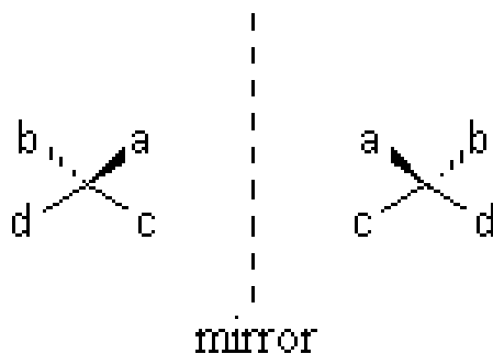
Fig. 3 Representation of enantiomers where a, b, c and d are different substituents.
