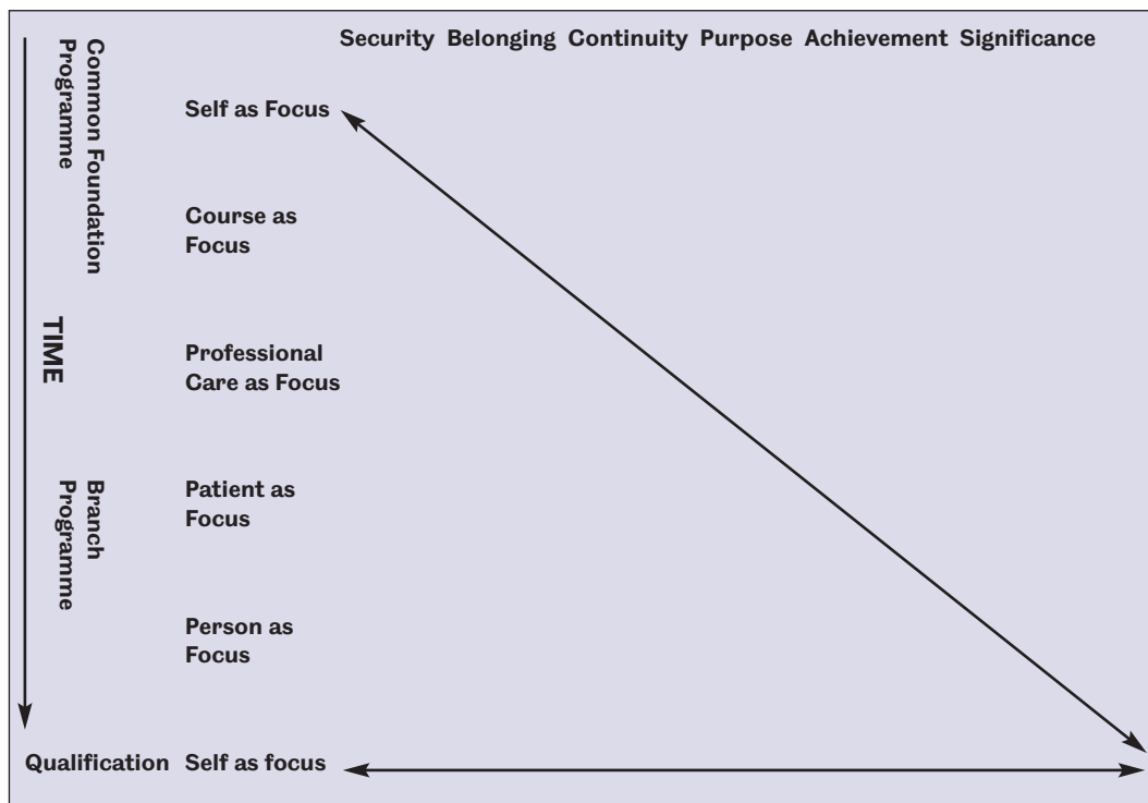
Figure 2: Influence of the Senses on student focus
