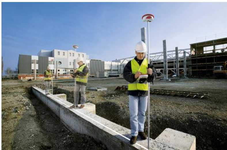
Figure 19: Kinematic GPS 'rover' gathering 3D surface data points (Kuker-Ranken Inc., no date)
