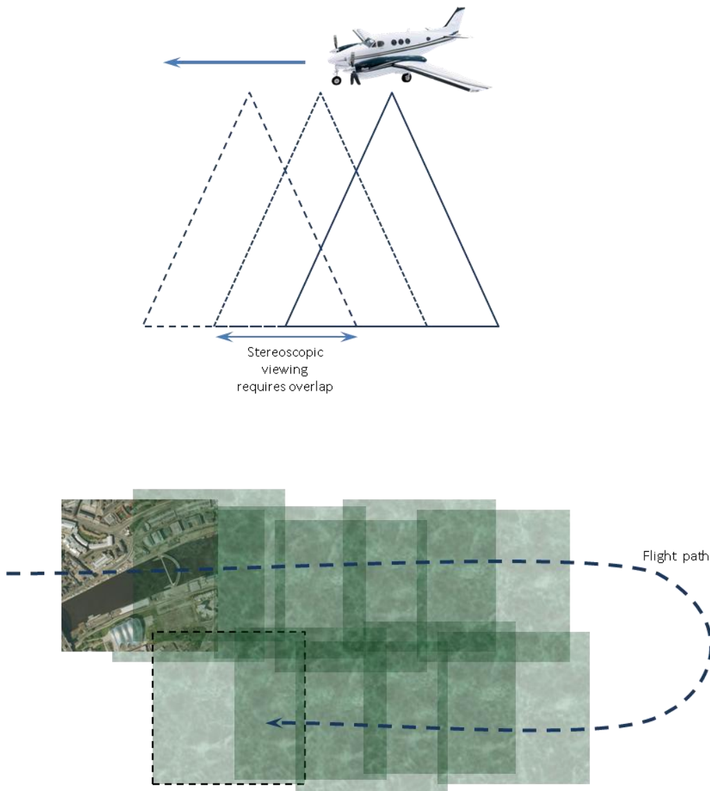
Figure 14: Production of large, stereoscopic aerial photographs requires a 60% forward overlap and 20% adjacent overlap (Gibson, 2000)
