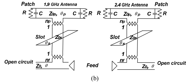
Fig. 6 (a) Physical structure of the antenna (b) Equivalent circuits of the antenna at the two frequencies
