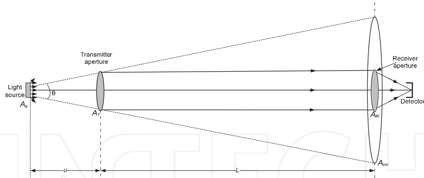
Fig. 7. Beam divergence
