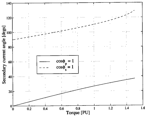
Fig. 9. Maximum power factor control angles at various torque levels
