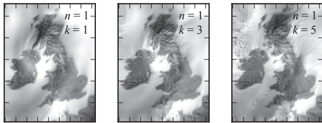
Fig. 1. Slices from the ensemble forecast output of the MOGREPS model, showing wind speed for scenario n = 1 . Black represents a wind speed of zero, and white represents speeds of at least 15 m/s. The forecast was carried out at 03:00 on 2nd Nov 2014, and k is measured from this time.
