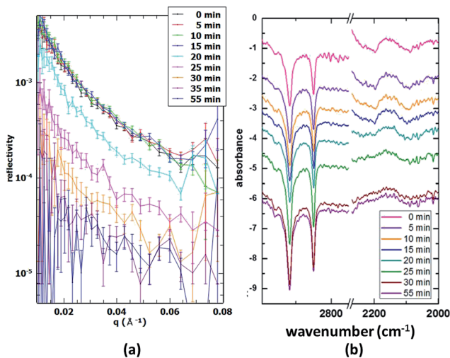
Fig. 4 Time-resolved NR and IRRAS data during the oxidation of a 1 : 1 mixed monolayer of stearic acid and deuterated oleic acid. Both CH and CD stretching vibrations are visible at about 2850–2920 and 2000–2200 \text{cm}^{-1} , respectively.
