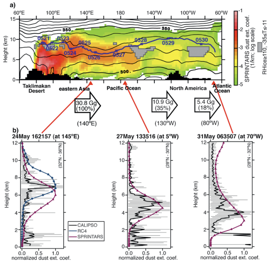
FIG. 9. (a) Vertical longitudinal cross sections of the Spectral Radiation-Transport Model for Aerosol Species (SPRINTARS)-simulated dust extinction coefficient along a Hybrid Single-Particle Lagrangian Integrated Trajectory model (HYSPPLIT) trajectory. Large arrows show horizontal dust fluxes at 140°E, 130°W, and 80°W estimated by SPRINTARS. The percentage in each bracket is the ratio of the dust amount to that exported to the Pacific through the 140°E meridian. (b) Normalized vertical profiles of the dust extinction coefficient measured by CALIOP (solid black lines) and simulated by RAMS/CFORS-4DVAR model system (blue lines with solid circles) and SPRINTARS (red lines with triangles), along CALIOP orbits. The uncertainty of the CALIOP retrievals is denoted (horizontal error bars).
