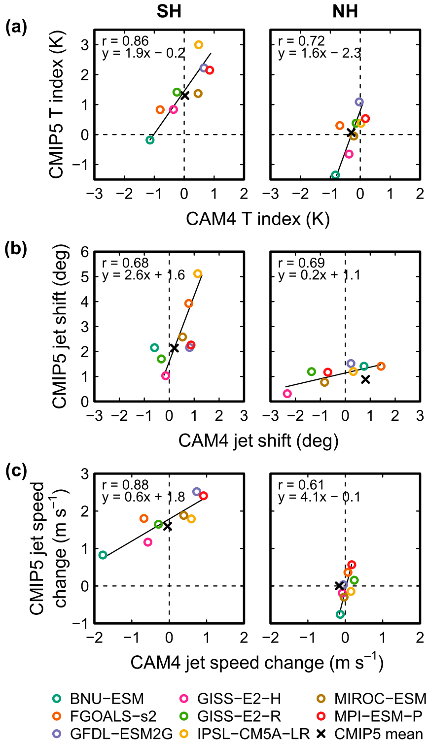
FIG. 8. Scatterplots of (a) temperature index, (b) jet shift, and (c) change in jet speed in CMIP5 abrupt4xCO2 simulations vs CAM4 ghost forcing experiments. The CAM4 results are the responses due to imposed albedo and cloud feedbacks. The jet shifts are defined as positive poleward. Orthogonal least squares regression lines are plotted, with the equation shown in the top-left corner of each panel.
