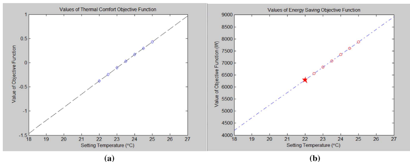
Fig. 10. Decision-making Outcomes in an Open Plan Office (PMV Model-Based BEMS).
