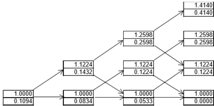
Figure 2.2: Procedure for valuing an American-style lookback options
