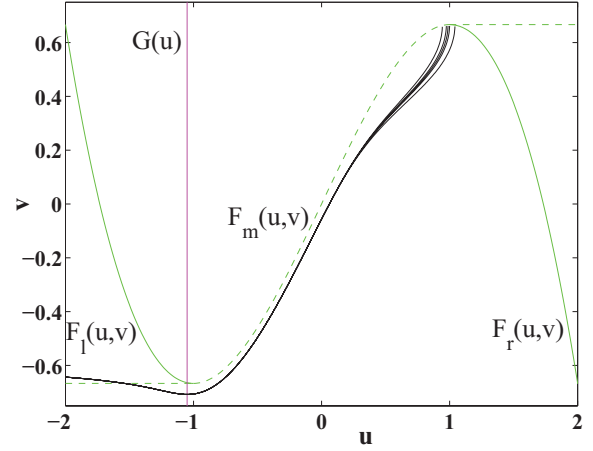
FIG. 2. (Color online) The boundary structures in the singular limit \epsilon \rightarrow 0 (dashed line) and for the finite value of \epsilon = 0.05 (solid lines) are shown in the u - v phase plane (dimensionless units). The nullcline G(u) and the branches F_l(u, v) and F_r(u, v) are shown by solid lines and the branch F_m(u, v) is shown by the dashed line. The trajectories for finite \epsilon correspond to solutions of an initial value problem, i.e., they were calculated by integrating Eq. (1) directly in time for specified initial conditions (u_0, v_0) : for the curves shown, u_0 = -3 and v_0 has been varied. The parameters of the FHN system (1) are a = 1.05 and \epsilon = 0.05 .
