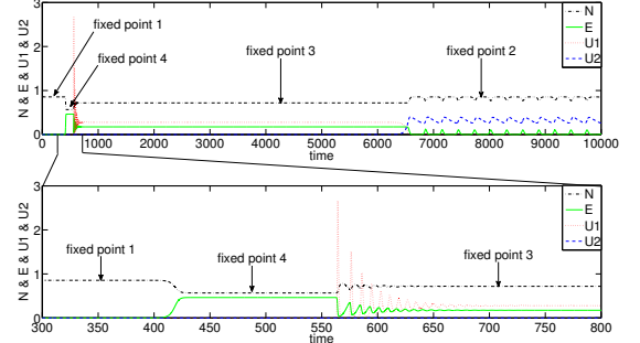
Figure 12. Time series of Fig. 2 in this paper, annotated in light of Fig.13.
