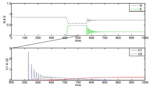
Figure 1. Upper panel: From overpowered H-mode to unstable L-mode then to T-mode. Lower panel: Transition to T-mode for U_1 and U_2 showing intersection at t \simeq 750 followed by energy reversal. The parameters are \nu_1 = 19 , \nu_2 = 1.01\nu_1 , \eta_1 = 0.12 , \eta_2 = 1.01\eta_1 , q = 0.47 , \rho = 0.55 , \sigma = 0.6 , \zeta = 1.7 .
