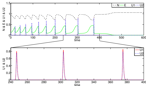
Figure 5. Upper panel: Collapse of limit cycle with positively correlated growth of pulses of U_1 and U_2 . Lower panel: Zoom in version from t = 240 to t = 400 . The parameters are \nu_1 = 19 , \nu_2 = 1.0001\nu_1 , \eta_1 = 0.12 , \eta_2 = 1.0001\eta_1 , q = 0.582 , \rho = 0.55 , \sigma = 0.6 , \zeta = 1.7 .
