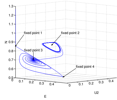
Figure 13. Phase plot of Fig. 2 in this paper.
