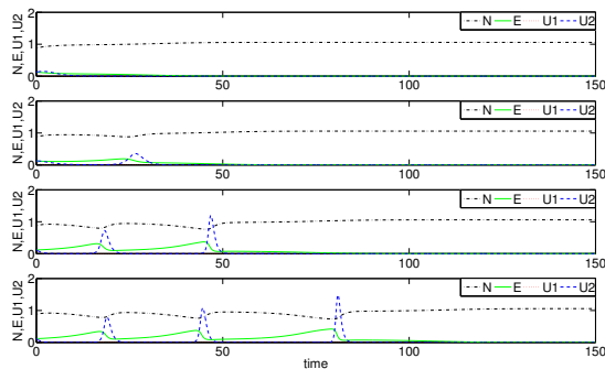
Figure 6. Evolution to the finite N attractor for different values of \eta_2 . Upper panel: \eta_2 = 0.05 . Middle upper panel: \eta_2 = 0.06 . Middle lower panel: \eta_2 = 0.10 . Lower panel: \eta_2 = 0.11 . The remaining parameters are the same: \nu_1 = 19 , \nu_2 = 1.001\nu_1 , \eta_1 = 0.12 , q = 0.582 , \rho = 0.55 , \sigma = 0.6 , \zeta = 1.7 .
