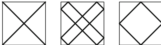
Figure 1: The sets M(0) , M(1/3) and M(1)
