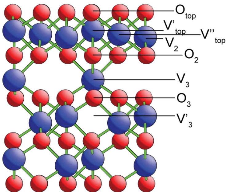
Fig. 9 Side view (viewed along [2\bar{1}10] ) of V_2O_3(0001) , showing modified form of the oxygen termination (the KSSN ..VV''V'O model) in which the V_2 half-metal layer moves up into the outermost buckled full metal layer (defined by the V'_{top} and V_2 half-layers) to become relabelled as V''_{top} . The simplified model shown here has all other interlayer spacings as in the bulk.
