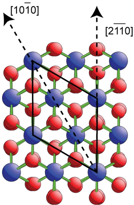
Fig. 4 Top view of the V_2O_3(0001) surface (with a half-metal termination) including a definition of the two principle azimuths in which the MEIS experiments were conducted. The full lines show the surface unit mesh that is also the base of the hexagonal 3D unit cell.
