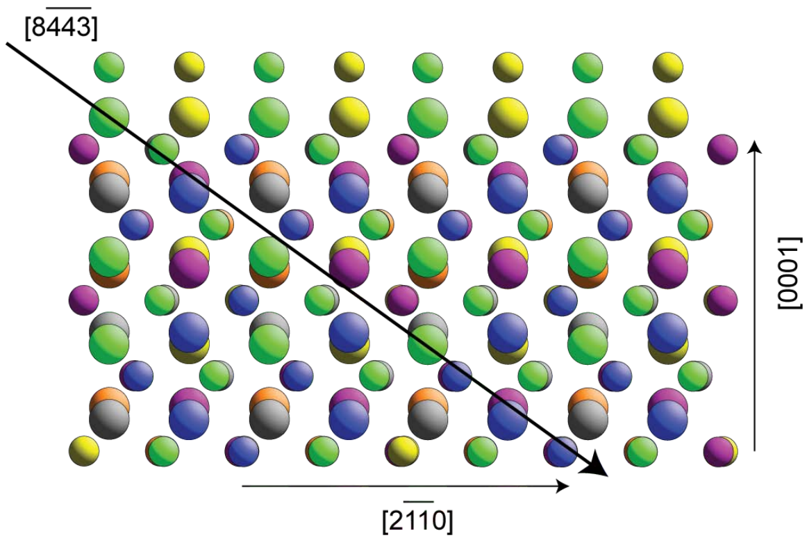
Fig. 6 Side view diagram of the four inequivalent V scattering planes (shown in different colours) for V_2O_3 in the [2\bar{1}\bar{1}0] azimuth, showing the incidence direction used. Larger balls represent V atoms, smaller balls represent O atoms. The O atoms in the bulk lie slightly out of the V atom planes, but may be expected to produce some shadowing and blocking.
