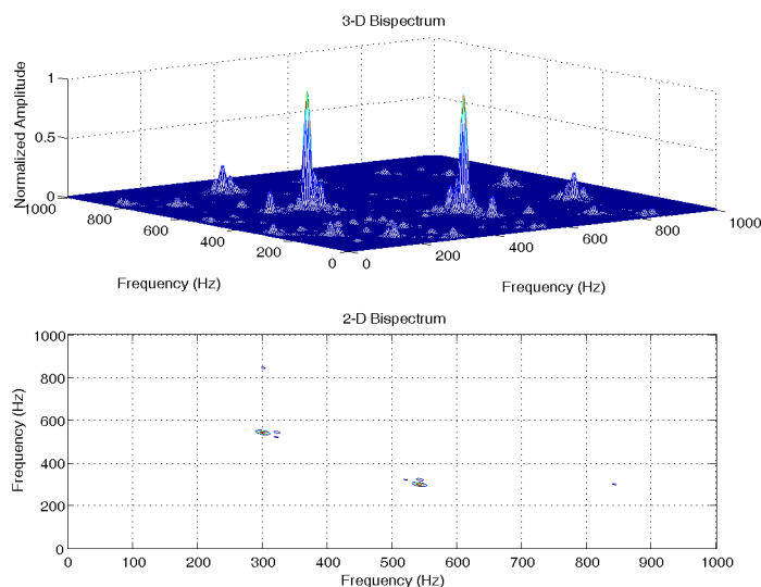
Figure 16 The vibration bispectrum of a healthy motor
