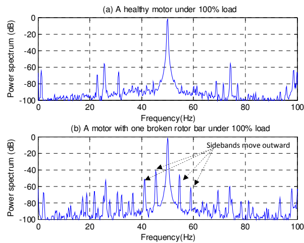
Figure 10 The stator current power spectra of induction motor without and with broken rotor bar fault under 100% load
