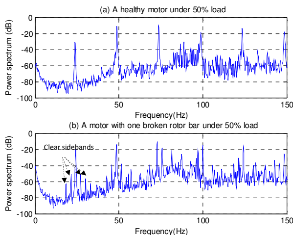
Figure 6 The vibration power spectra of induction motor without and with broken rotor bar fault under 50% load
