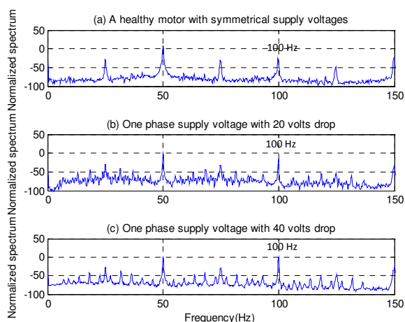
Figure 12 The stator current power spectra of induction motor without and with 20V and 40V drop of one phase voltage
