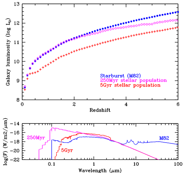
FIG. 17.— Top panel : SERVS faintest galaxy to be detected, in units of solar luminosities (integrated luminosity from the optical to the far-IR: 0.1\mu\text{m} – 1\text{mm} ) at a given redshift. Three Spectral Energy Distribution (SED) models are considered here and shown in the bottom panel . The three SEDs consist of an M82-like starburst galaxy (in blue), a 250 Myr stellar population (magenta) and a 5 Gyr stellar population (red), scaled to the same 3.6\mu\text{m} rest-frame. SERVS can detect L^* galaxies out to z \sim 4 , and 0.1L^* out to z \sim 1 . At redshift 5, a starburst galaxy of luminosity \sim 10^{12} L_{\odot} could potentially be detected.
