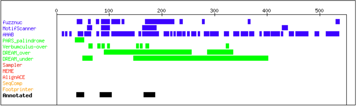
Figure 2. The predictions of the algorithms over a stretch of 550 base pairs in a yeast promoter region. The last row shows the actual position of the known binding sites
