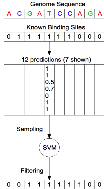
Figure 3. At each position in the yeast genome sequence we have an annotation and 12 algorithmic predictions of that annotation. We train an SVM to produce the annotation given the 12 algorithmic predictions.
