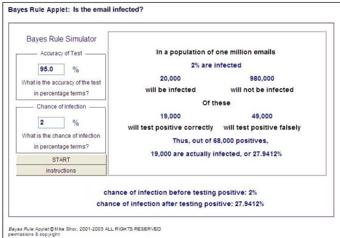
Figure 2. A simple application of Bayes’ theorem, adapted and reproduced with permission from Shor, Mikhael (2005), “Bayes Rule Applet”, Game Theory .net , http://www.gametheory.net/Mike/applets/Bayes/Bayes.html .
