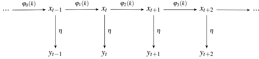
Figure 6: A graphical representation of mixture latent markov
