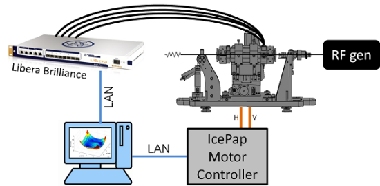
Figure 7: Schematic of lab setup and equipment connectivity for wire scanning the BPMs.
