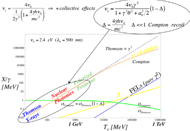
Figure 1: Operating Diagram for Thomson/Compton Sources, showing the elastic (no-recoil) Thomson regime for X-rays and the small recoil regime typical of Compton Sources for Nuclear Photonics. The deep Compton regime, dominated by recoil effects and typical of \gamma - \gamma collider is also shown, together with the behavior of the recoil parameter \Delta and the Compton cross section decrease together with increasing \Delta . The enhancement of the formula for the frequency of the back-scattered photon is also shown, taking into account the red-shift effects due to scattering angle \theta and non-linear multi-photon effects generated by laser field intensity (represented by the laser parameter \alpha_0 ).
