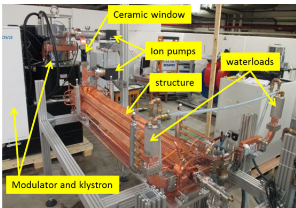
Figure 9: C-band structure under high power test.
