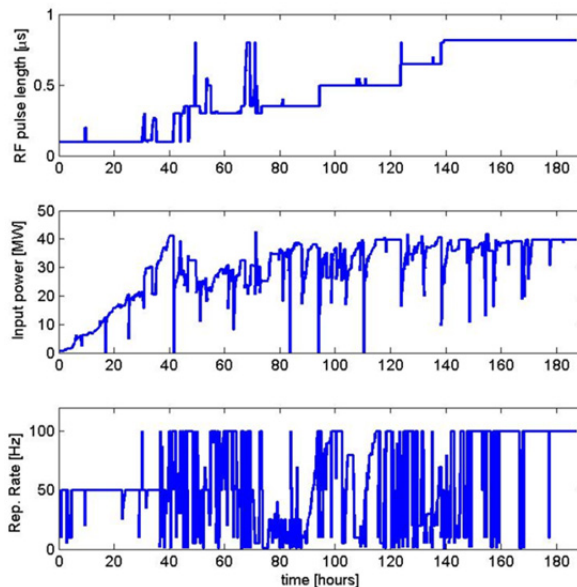
Figure 10: Behavior of the RF Pulse length, input power and repetition rate as a function of time during the high power test of the C-band structure.
