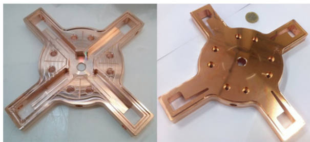
Figure 1: Picture of machined cell.
