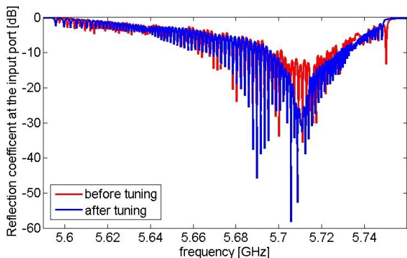
Figure 8: reflection coefficient at the input port before and after the tuning.
