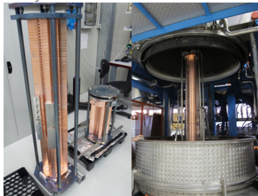
Figure 4: (Left) two half structures before brazing; (right) full assembled structure in the LNL-INFN oven.
