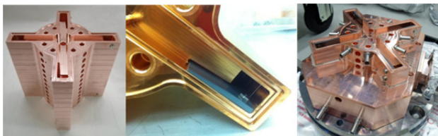
Figure 3: From the left: Twelve cell module, detail of the SiC absorber fixed inside the module, input coupler.
