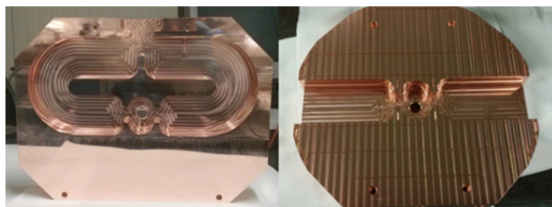
Figure 2: Machined input and output couplers.
