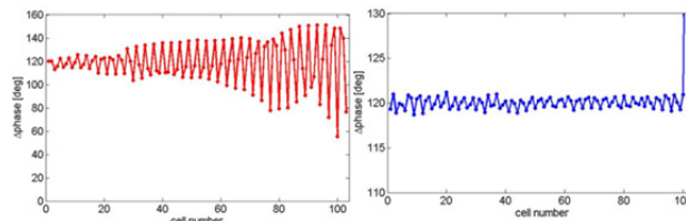
Figure 7: Phase advance per cell before (left) and after (right) tuning.
