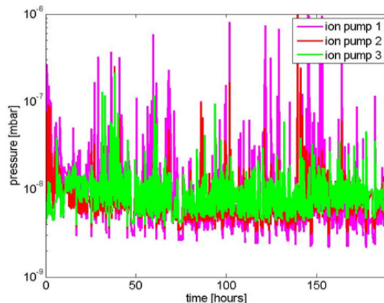
Figure 11: Vacuum pressure as a function of the conditioning time.
