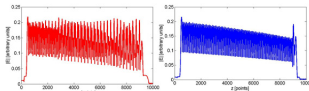
Figure 6: magnitude of the accelerating field before (left) and after (right) the tuning.
