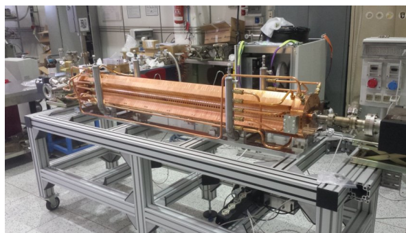
Figure 5: Full C-band structure.
