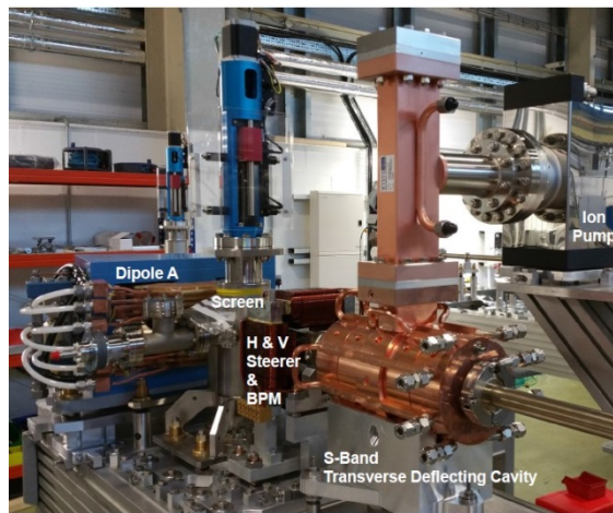
Figure 7: S-Band transverse deflecting cavity.
