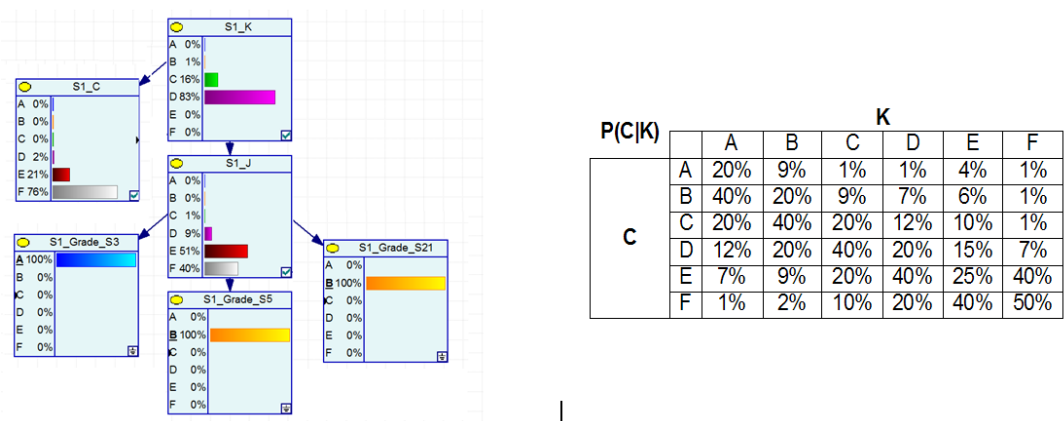
Figure 1. (left) A sample fragment of the BN in OpenAnswer, showing the individual sub-network of student S1. K and J are stochastic variables computed during the network maintenance. C , the correctness of the answer given by the student S1, is a stochastic variable as well. On the contrary, the (three) evaluations given by this student (to the answers of peers S3, S5, S21) are just fixed: their values, together with those given by the other peers to the same answers, will concur in composing the distribution of probability for the related C values. (right) A sample CPT. It is the P(C|K) conditional probability table used in the experiments. It was devised based on experience and is fixed in the system, as well as for the other CPTs we used in this study. We discuss in the conclusions section about the possibility to learn the CPTs from previous experience with the classroom.
