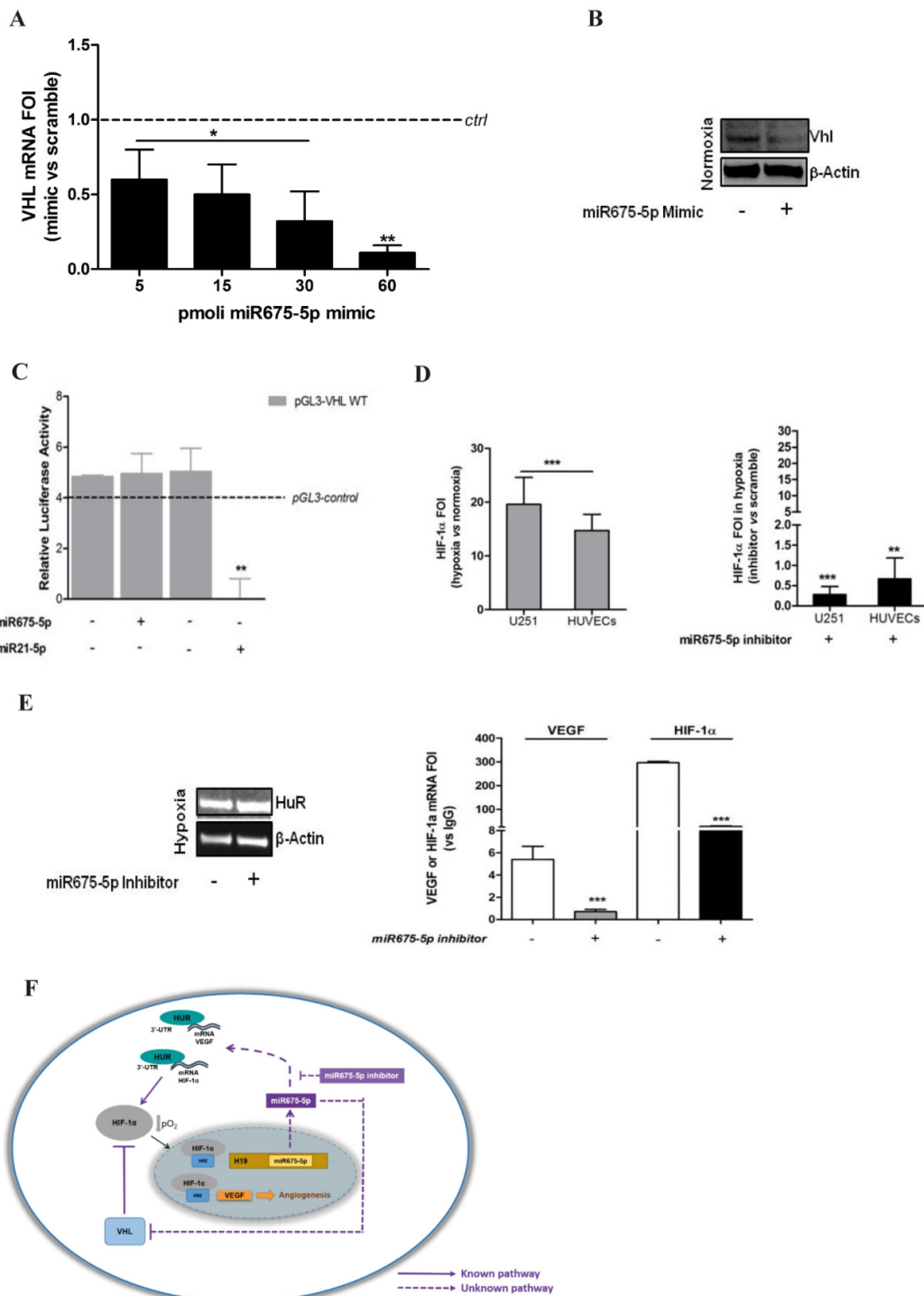
Figure 5: miR675-5p regulates HIF-1 \alpha mRNA stability by VHL/HuR axis. (A) Real-time PCR for VHL was done on U251 cells 18h after transfection with 5pM, 15pM, 30pM and 60pM of miR675-5p mimic. The dashed line indicates the control sample (scramble-treated). Values are presented as the mean \pm SD. Mimic vs scramble * p < 0.05 ; ** p < 0.01 . (B) Western Blot for VHL and \beta -actin from U251 cells transfected with miR675-5p mimic (5pM) or scramble negative control. (C) Expression of VHL-regulated miRNA was validated by Luminescence assay kit, a secondary reporter was used for transfection normalization. Data are expressed as Relative Luciferase Activity in pGL3-pVHL-WT construct transfected with miR675-5p or miR21-5p and their relative scrambles. pGL3-control is represented as dashed line. The mean \pm SD of three independent experiment is shown, and each sample was assayed in triplicate. (D) Left panel: Real-time PCR for HIF-1 \alpha performed on U251 and HUVEC cells 6 hours post-hypoxia. Data were normalized for \beta -actin, and \Delta\Delta C_t is expressed as fold of induction (FOI) of HIF-1 \alpha in hypoxia vs normoxia. Right panel: Real-time PCR performed on U251 and HUVEC cells 6 hours post-hypoxia and after miRNA675-5p inhibitor transfection. Data were normalized for \beta -actin, and \Delta\Delta C_t is expressed as fold of induction (FOI) of HIF-1 \alpha in hypoxia in inhibitor vs normoxia. (E) Left panel: Western Blot for HuR and \beta -actin from U251 cells transfected with miR675-5p inhibitor (5pM) or scramble negative control after 6h of hypoxia. Right panel: RNA-immunoprecipitation for HuR. Real time PCR for VEGF and HIF-1 \alpha were performed starting from HuR co-immunoprecipitated RNA in different culture conditions. Ct value was normalized to the Input RNA Ct value. Data are expressed as fold enrichment above the input percentage and presented as the mean \pm SD. Inhibitor vs scramble negative control *** p < 0.001 . (F) Molecular mechanism of miRNA 675-5p in hypoxia condition. The dashed line indicates our experimental results.
