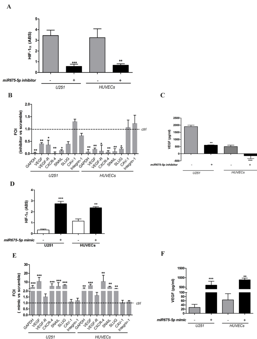
Figure 2: Gain and loss of function suggests a critical role of miR675-5p on hypoxia modulation. (A) ELISA for HIF-1α nuclear level in U251 and HUVECs transfected with miR675-5p inhibitor and exposed to hypoxia for 6h. Data are expressed as ABS values at 450nm. (B) Real-time PCR from U251 and HUVECs exposed to hypoxia after miR675-5p inhibitor or scramble control transfection. Data were normalized for β-actin and ΔΔct is expressed as fold of induction (FOI) of indicated genes after inhibitor transfection compared to scramble control (dashed line). (C) ELISA assay for VEGF level in supernatant from both cell lines transfected with miRNA inhibitor or negative control and exposed to hypoxia for 6h. Data are expressed as pg/ml of soluble VEGF. Values are presented as the mean ± SD. Inhibitor vs scramble * p<0.05; **p<0.01; ***p<0.001. (D) HIF-1α nuclear level analyzed by ELISA assay in U251 and HUVEC cells after 18h of miR675-5p mimic transfection in normoxia. Data are expressed as ABS values at 450nm. (E) Real-time PCR performed on U251 and HUVEC cells after miR675-5p mimic-transfection. Data were normalized for β-actin, and ΔΔct is expressed as fold of induction (FOI) in cells transfected with mimic compared to control (dashed line). (F) ELISA assay for VEGF level in supernatant from both cell lines 18h after mimic transfection. Data are expressed as pg/ml of soluble VEGF. Values are presented as the mean ± SD. Mimic vs scramble * p<0.05; **p<0.01; ***p<0.001.
