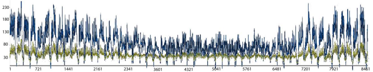
Fig. 6. Annual heat losses trends ante and post operam.
