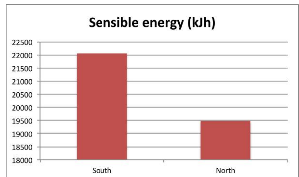
Fig.5 Heat loss comparison between south and north exposed thermal zones.
