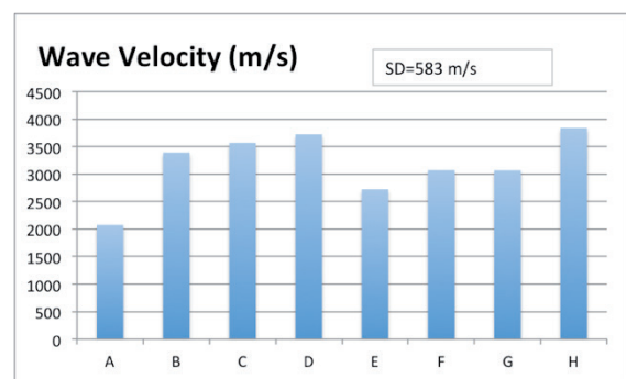
Fig. 17 First-floor slab Sonic Test chart results.
