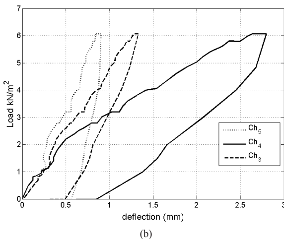
Fig. 10 (a) Positions of displacement transducers and the water dam during the loading test, a = 3.55 m, b = 2.27 m, c = 6.30 m, d = 5.80 , e = 0.50 m. (b) Load-displacement diagrams for the three transducer recordings.
