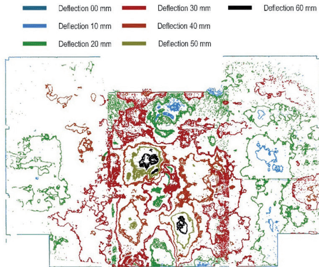
Fig. 15 First-floor slab deflection.
