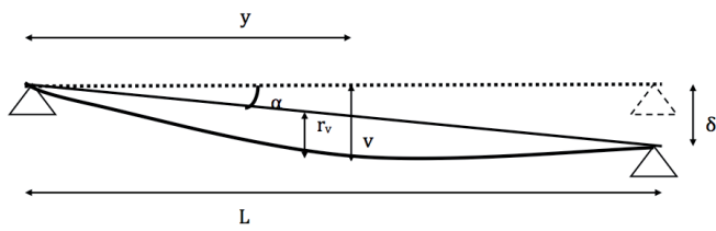
Fig. 14 Scheme of beam constraint displacement.
