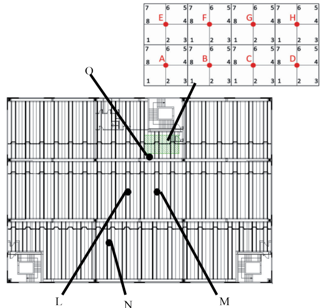
Fig. 16 First floor slab Sonic Tomography and ultrasound test positions.
